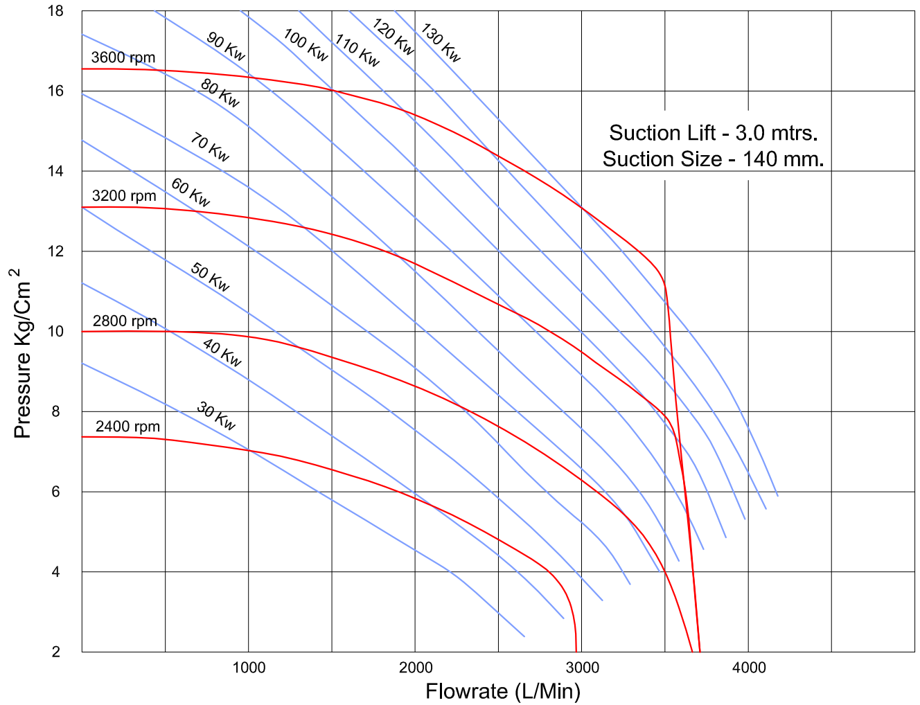
Typical Low Pressure Performance of MFV MP 1030
